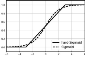
Fig. 4. Comparison between Sigmoid and hard-Sigmoid functions.
